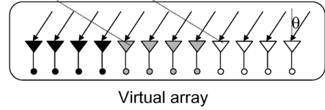
Fig. 2. Virtual array corresponding to the MIMO radar in Fig. 1.
