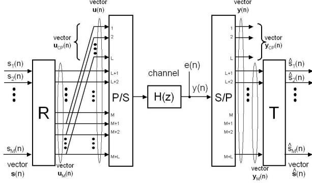
Fig. 1. A typical cyclic prefix system
