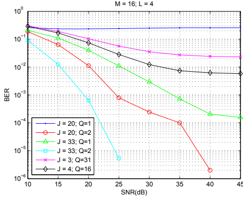
Fig. 3. Bit error rate performance for static channels.
